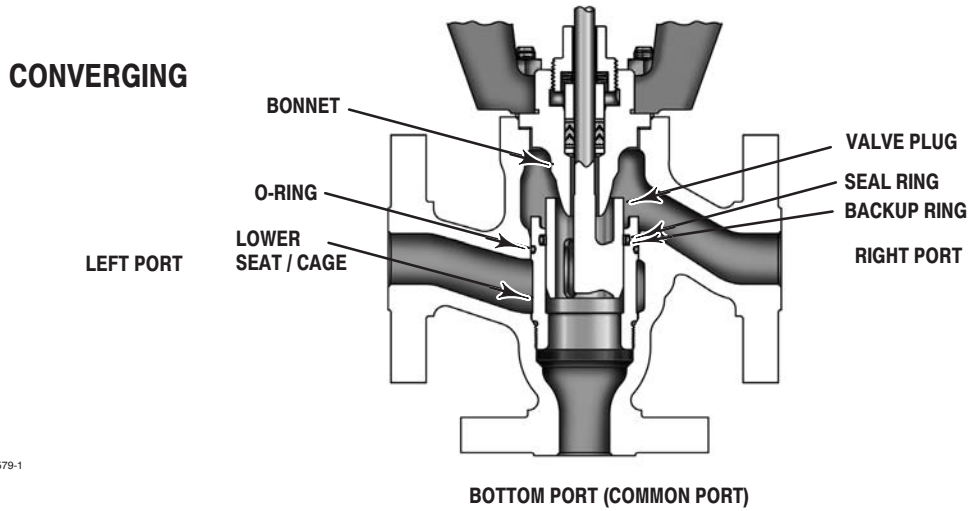
Figure 10. Bottom Port Common Construction Details for Converging Constructions
