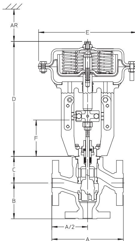
Figure 16. Fisher® GX 3-Way Dimensions (also see table 13)
