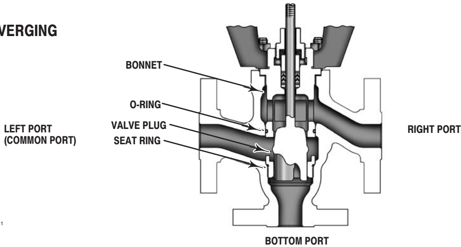
Figure 4. Side Port Common Construction Details for Diverging Constructions
