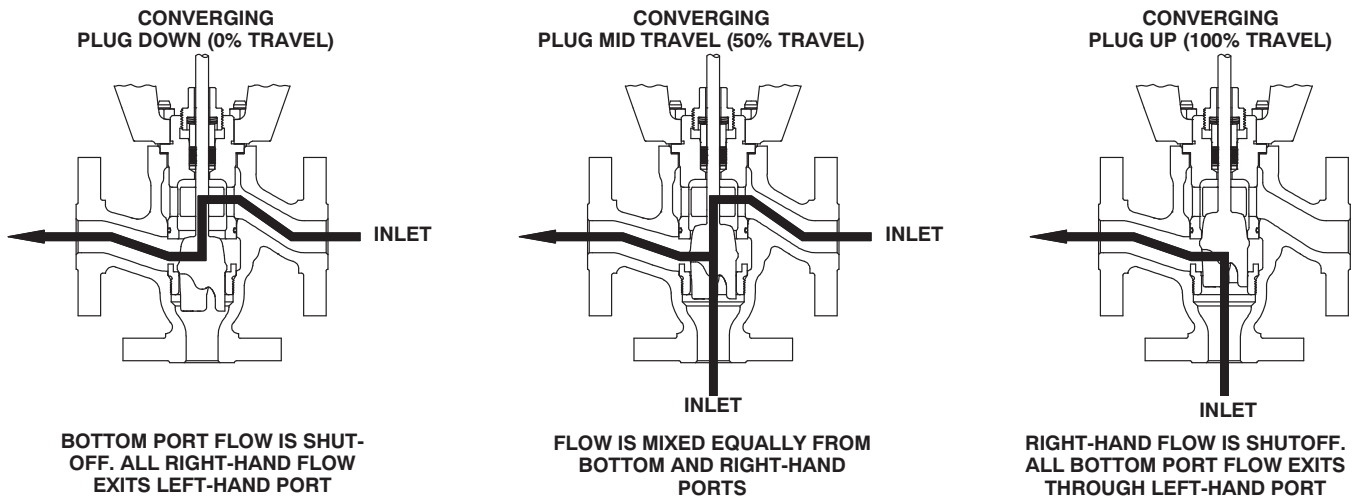
Figure 7. Fisher® GX 3-Way Flow Directions for Side Port Common Converging Constructions
