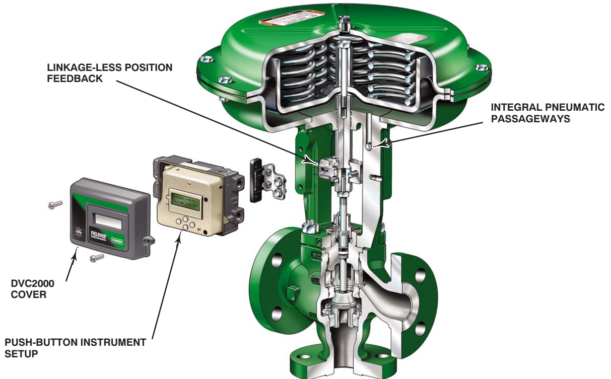
Figure 3. Fisher® GX 3-Way and DVC2000 Digital Valve Controller
