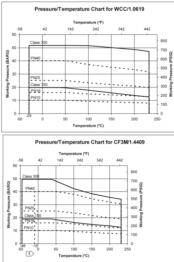
Figure 13. Material Pressure/Temperature Curves
